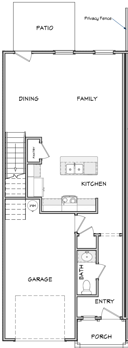
MAIN LEVEL
