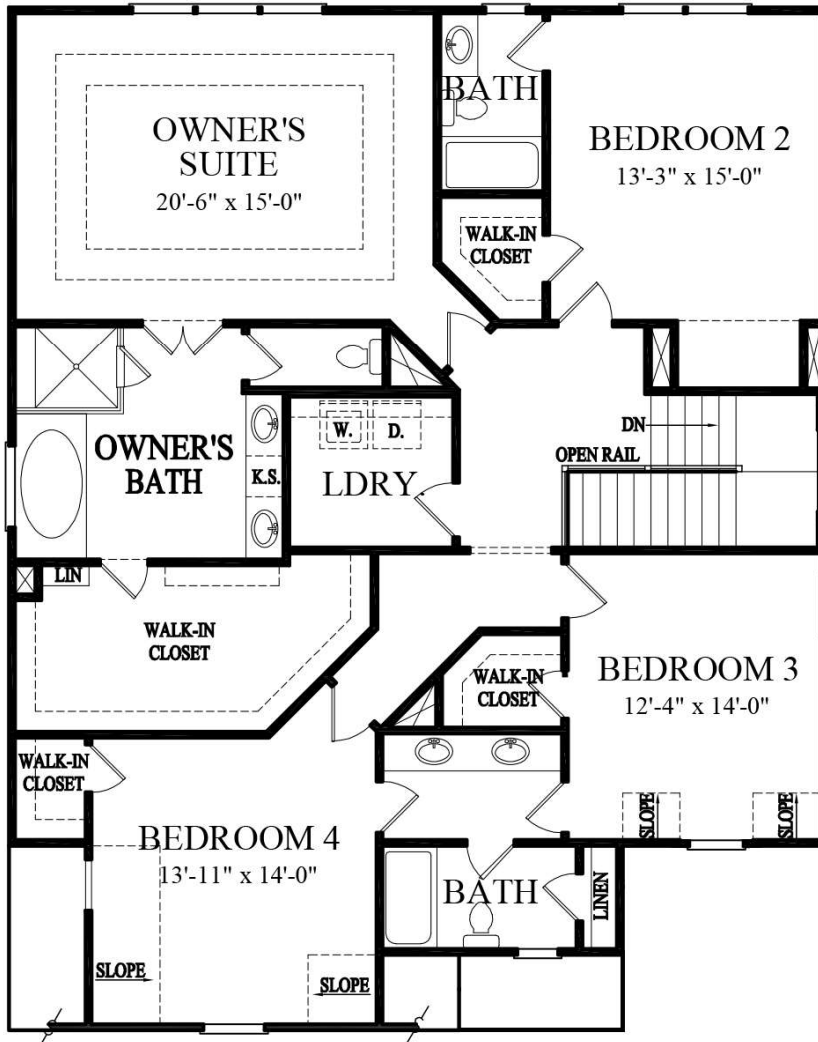
SECOND FLOOR
