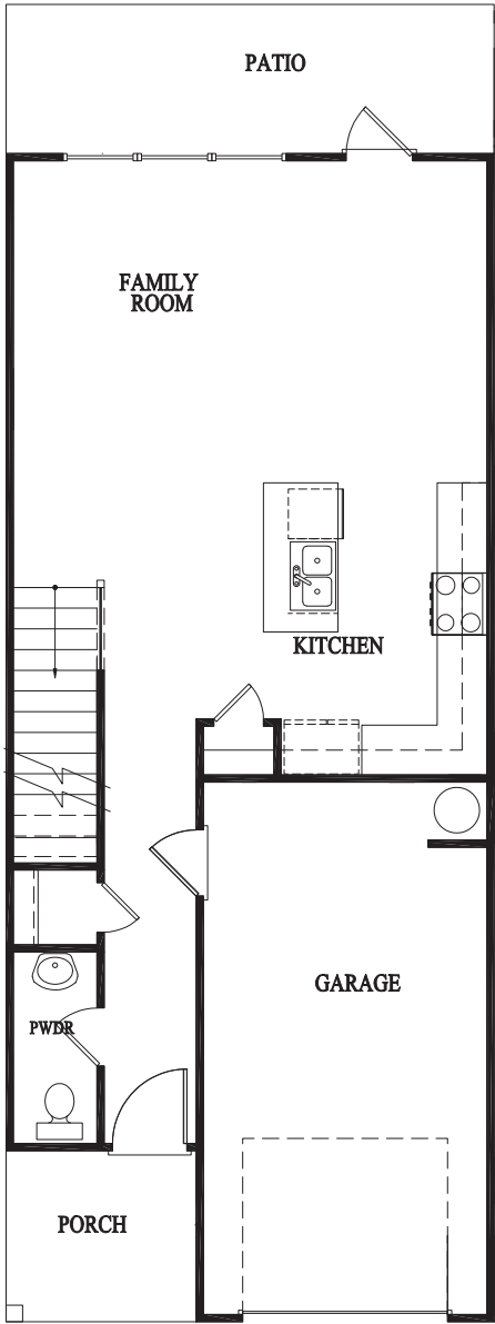
FIRST FLOOR
