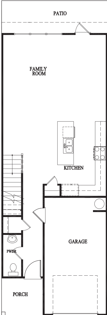
FIRST FLOOR
