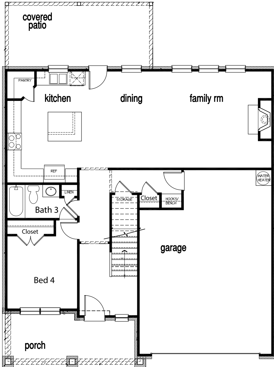
FIRST FLOOR
