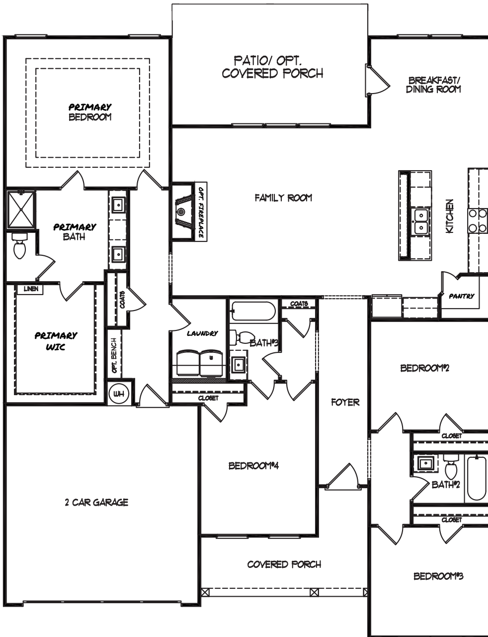
MAIN FLOOR
