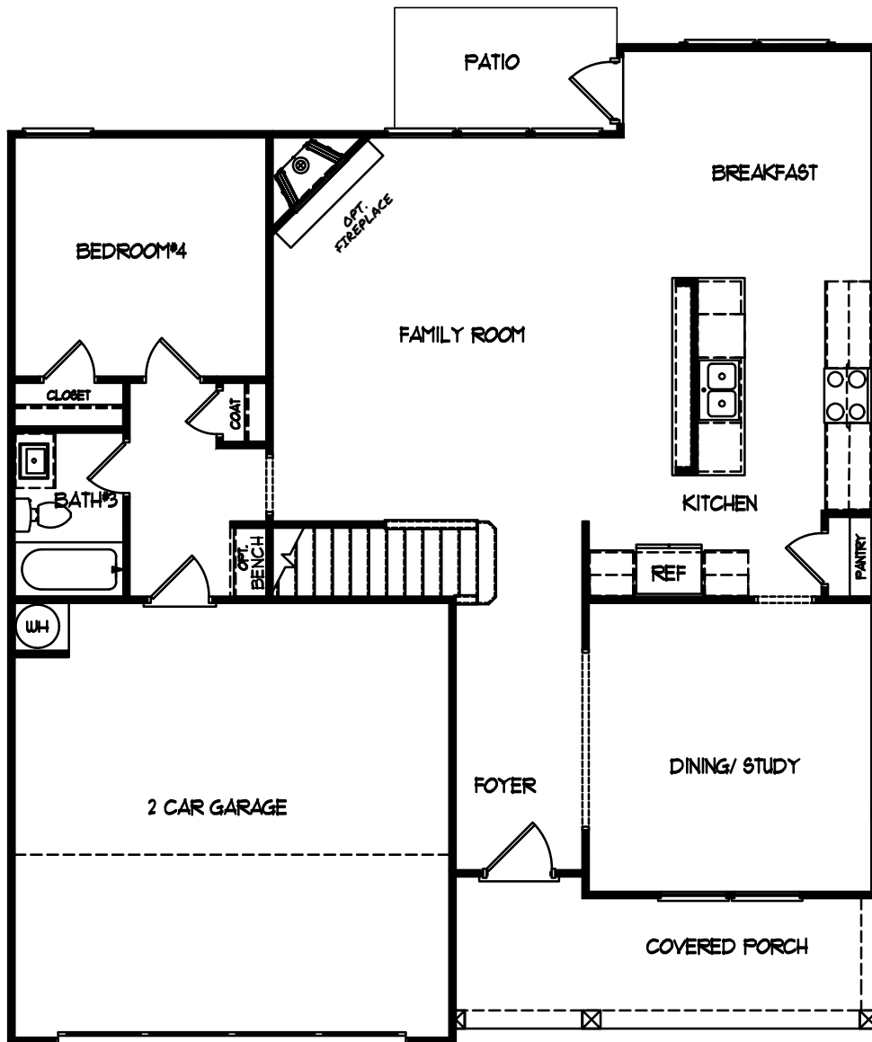
MAIN FLOOR
