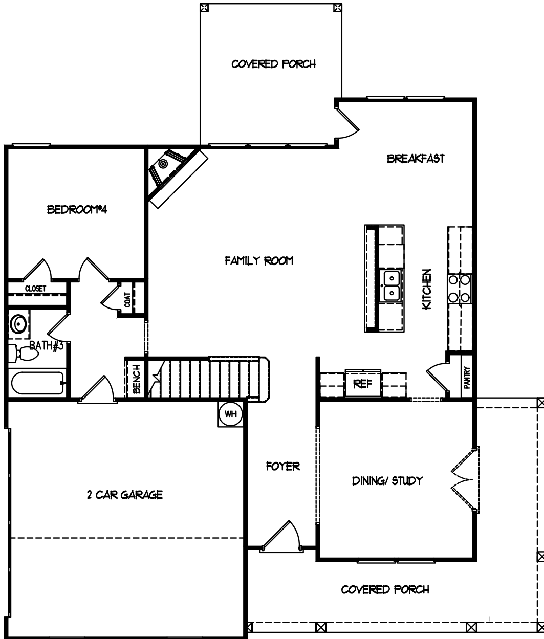
MAIN FLOOR
