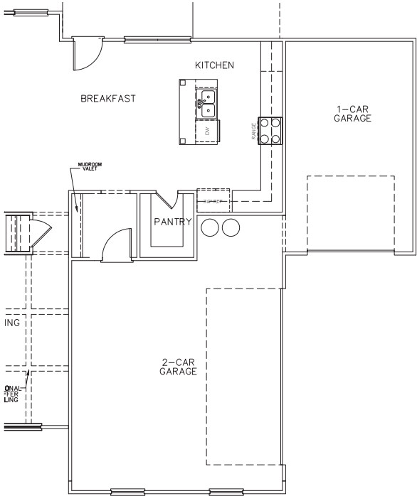
OPTIONAL 3 RD CAR BOLT SIDE ENTRY
