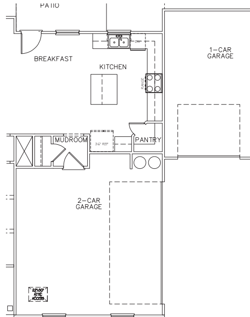
OPTIONAL 3 RD CAR BOLT SIDE ENTRY
